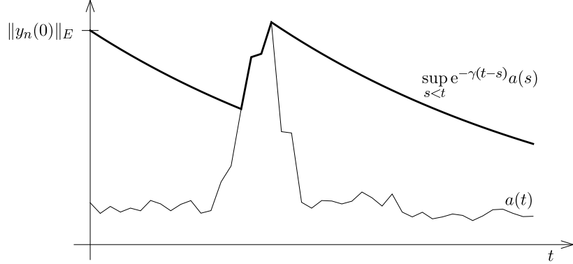
Figure 1: This picture illustrates the a-priori bound on \|y_n\|_E obtained in the proof of Theorem 2.6. Whenever \|y_n(t)\|_E is above a(t) = C(1 + \|z(t)\|_E)^N it decays exponentially. Therefore the thick line is an upper bound for \|y_n\|_E .
